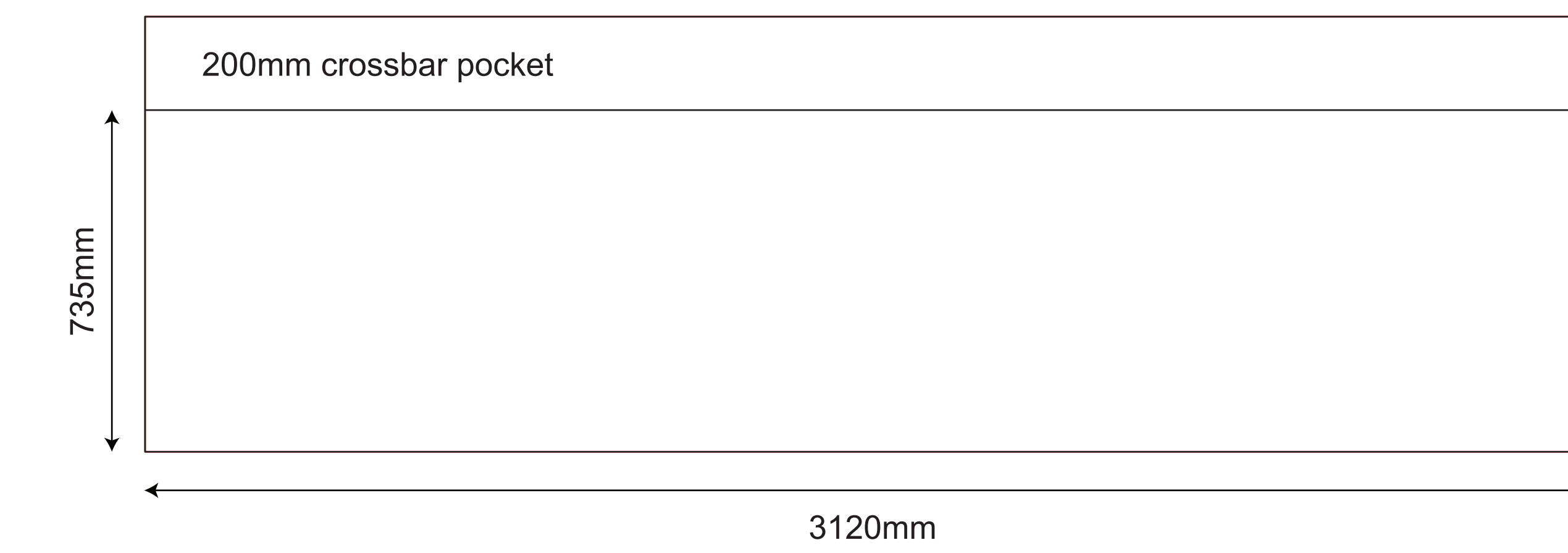
INSIDE OF THE GAZEBO - BACK SIDE - half wall
